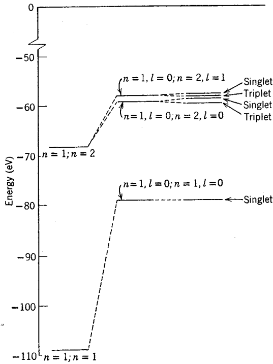
Figure 9-7 The low-lying energy levels of helium. Left: The levels that would be found if there were no Coulomb interaction between its electrons. Center: The levels that would be found if there were a Coulomb interaction but no exchange force. Right: The levels that would be found if there were a Coulomb interaction and an exchange force. These levels are in excellent agreement with the experimentally observed levels shown on the right in Figure 9-6.
