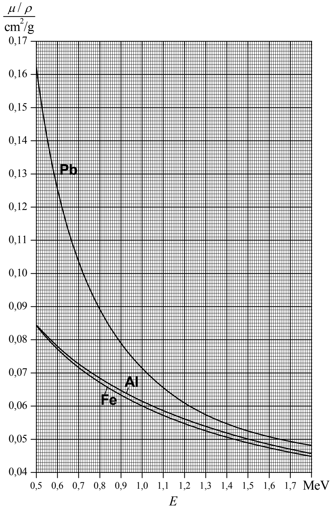
Fig. 16. Dependences of the mass attenuation coefficient of gamma radiation in lead, iron and aluminum on the photon energy (from http://atom.kaeri.re.kr/cgi-bin/w3xcom )
